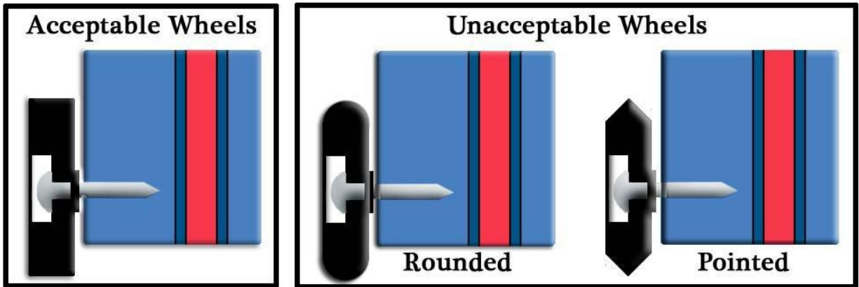
Figure A: Acceptable and Unacceptable Wheels
